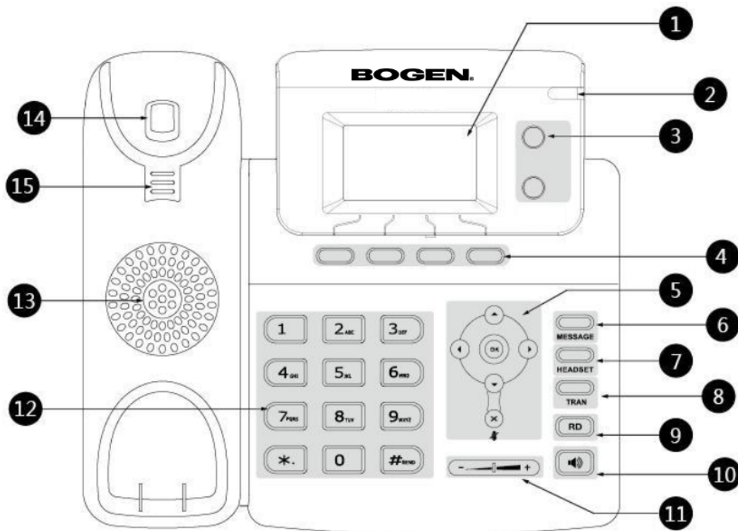
Figure 1-1, Hardware Components
